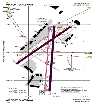
Digital NOTAMs on Airport Diagram
