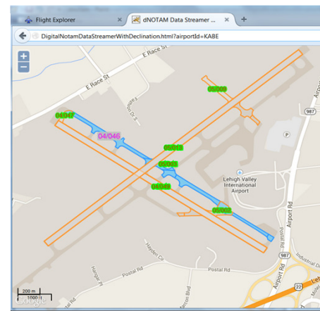
Digital NOTAMs on Moving Map
